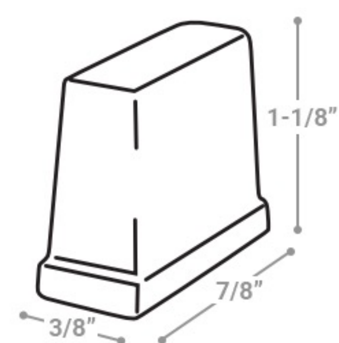
Half-sized cube dimensions
