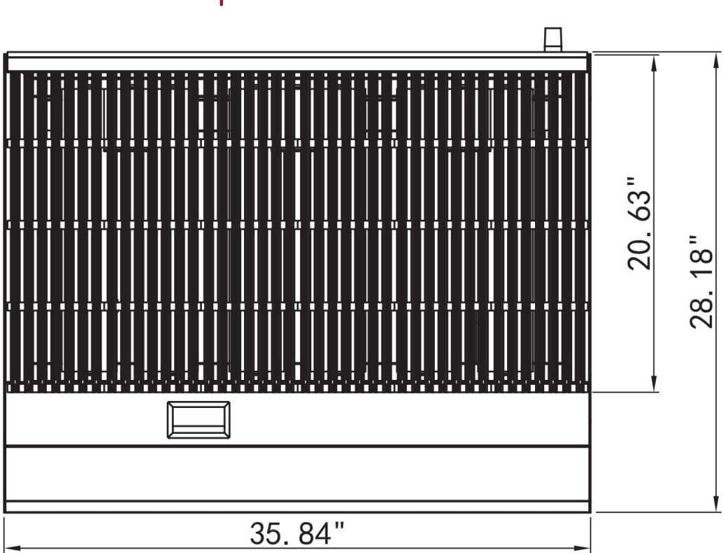
MBR36 - Top View
