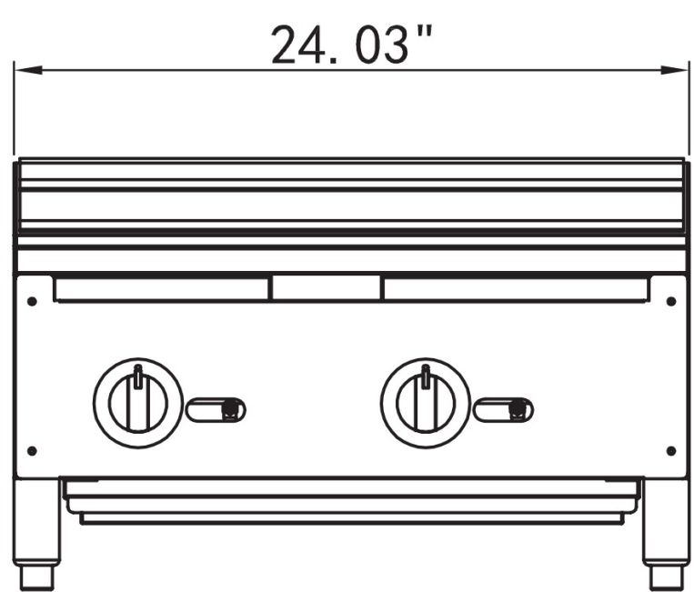
MBR24 - Front View
