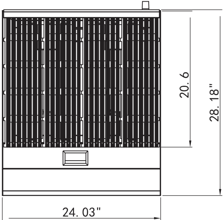
MBR24 - Top View
