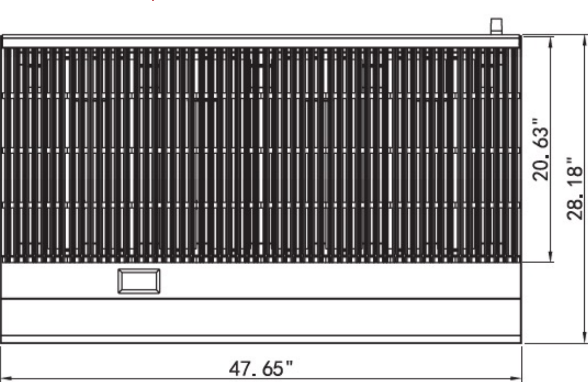
MBR48 - Top View
