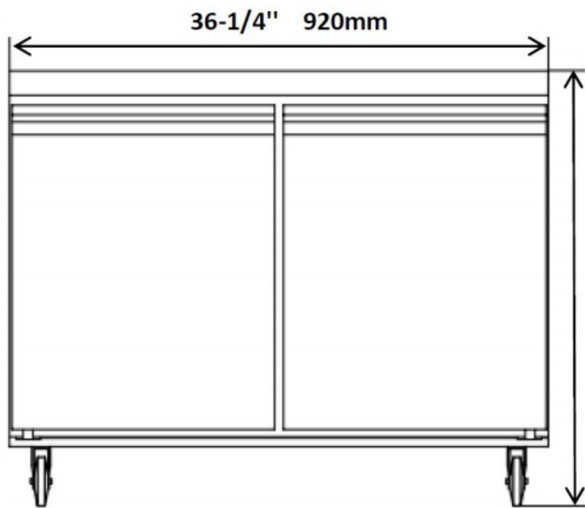
Front View
