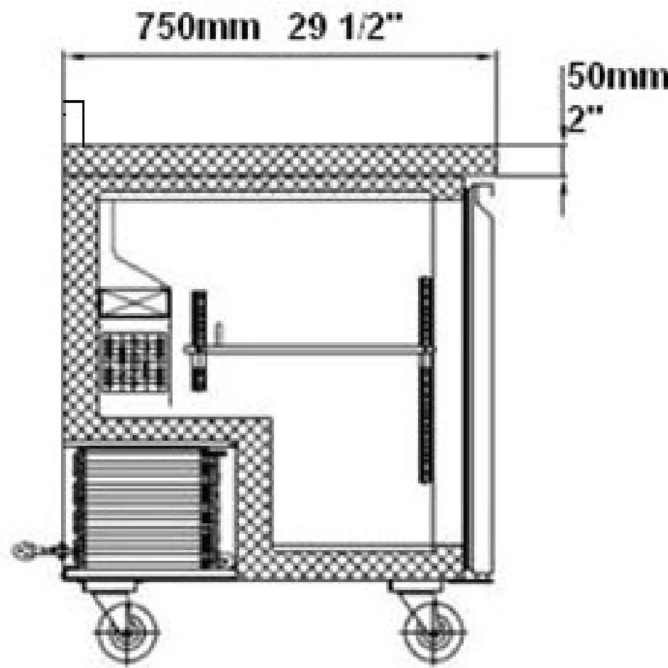
Side View
