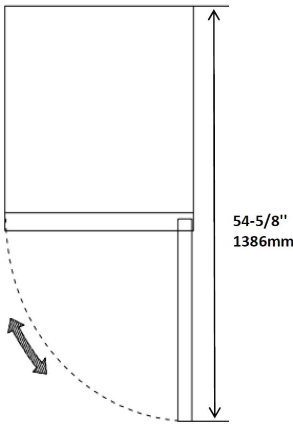
Top View
