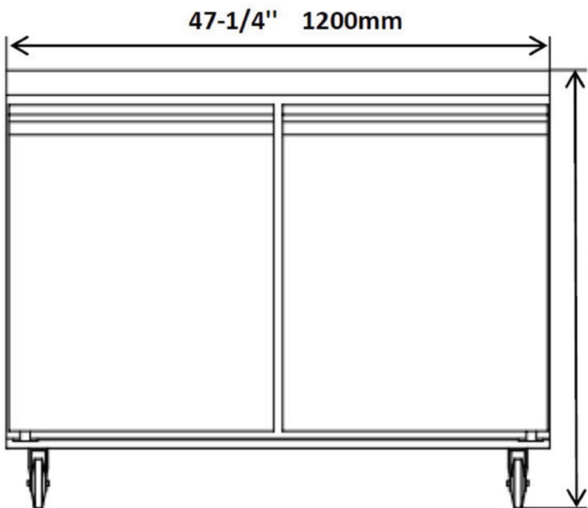
Front View
