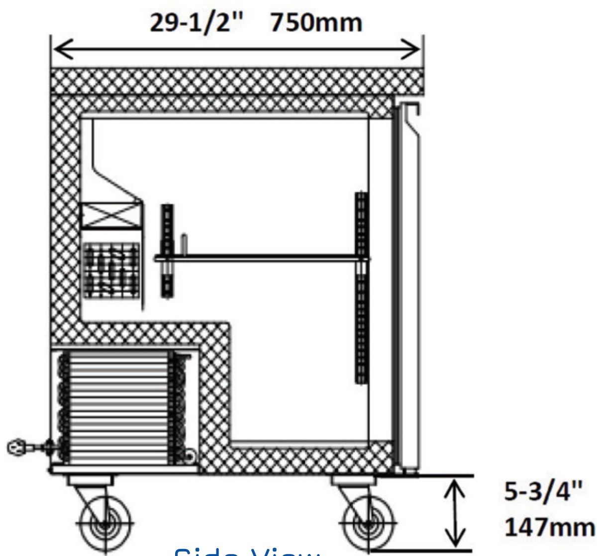
Side View
