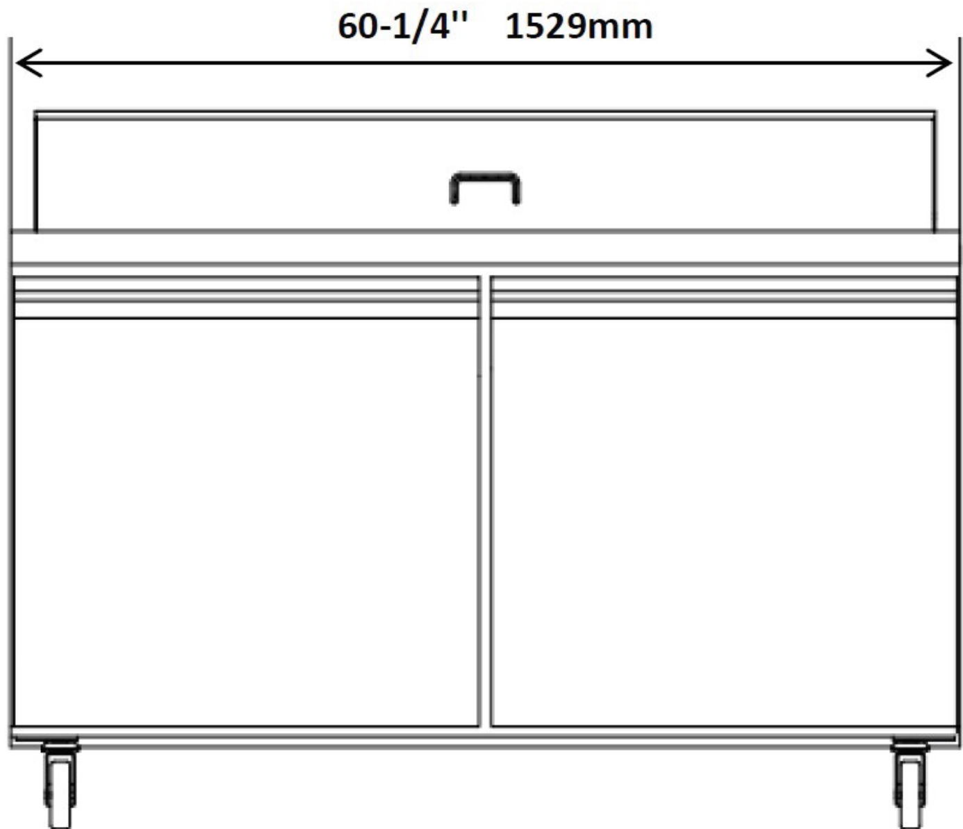
Front View
