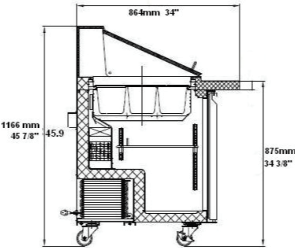
Side View
