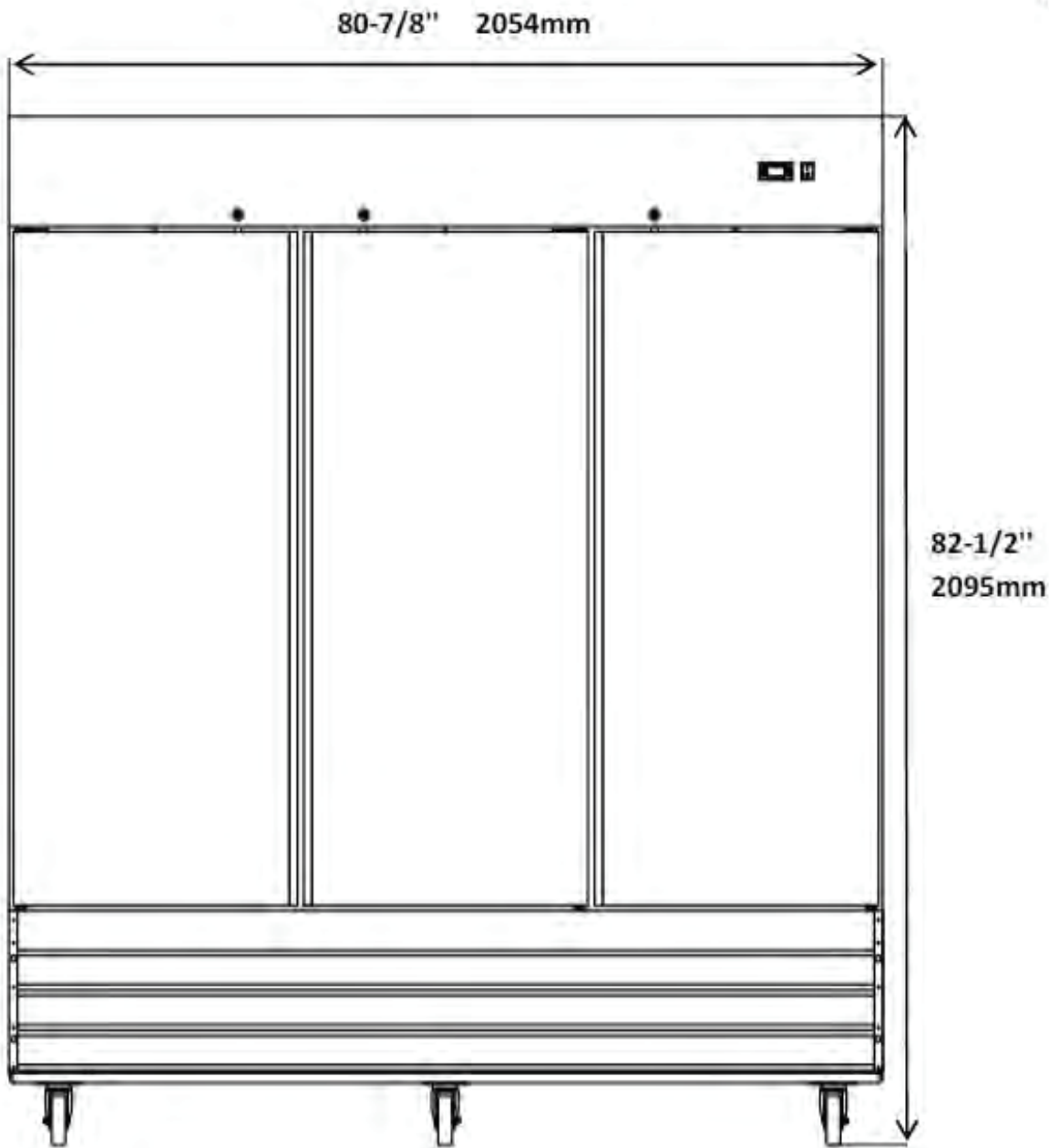
Front View
