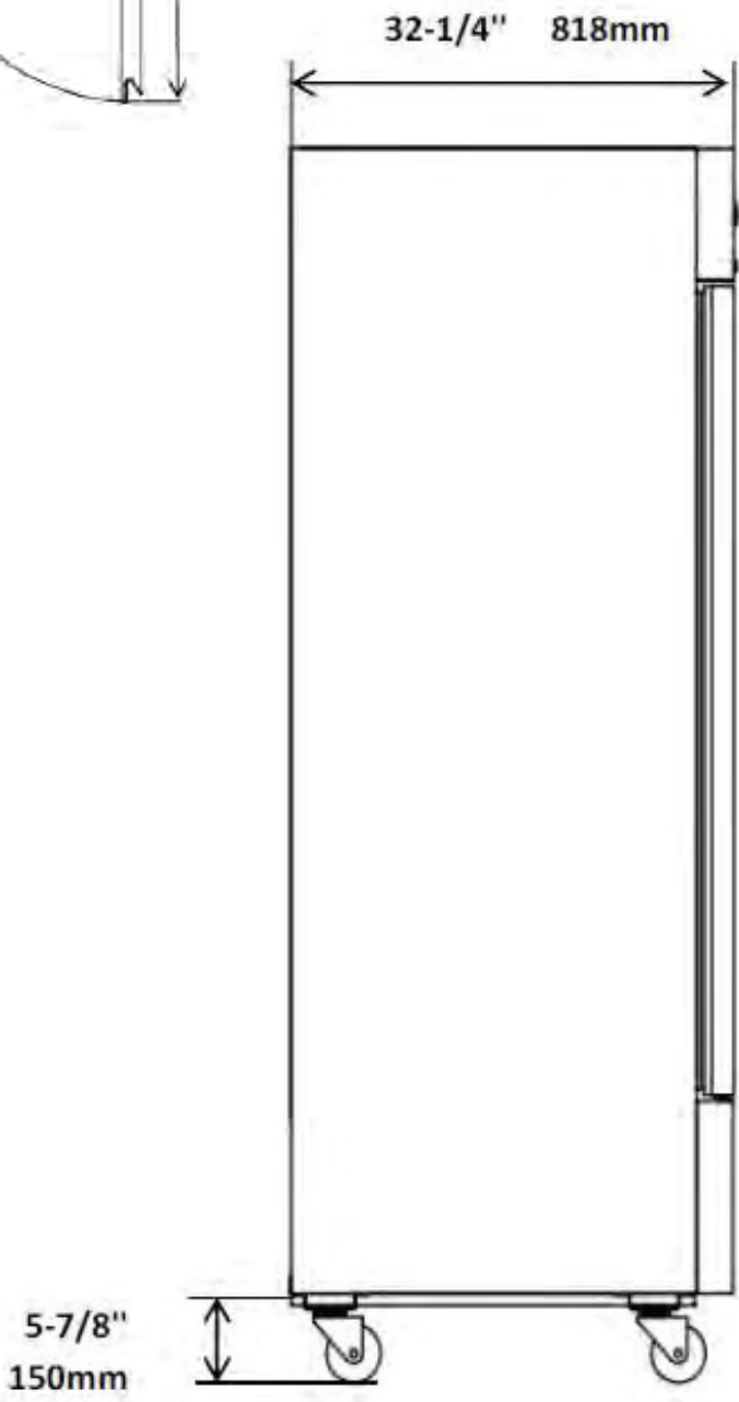
Side View
