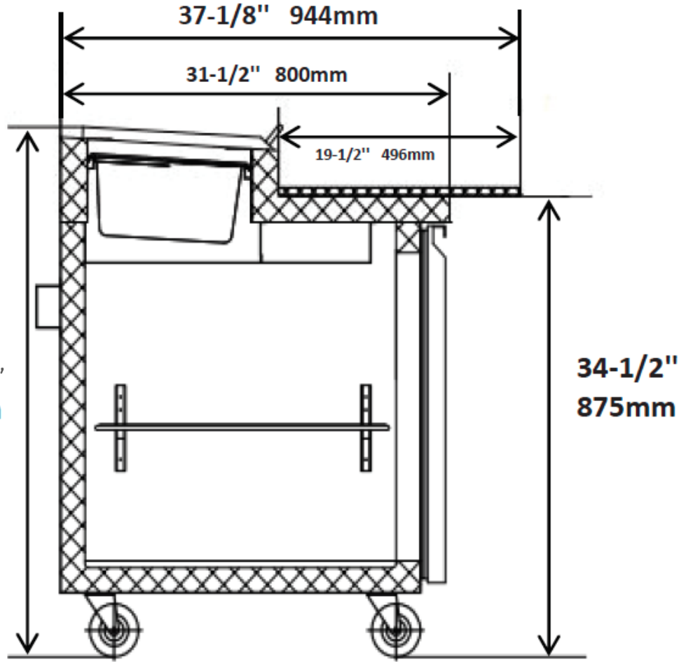
Side View
