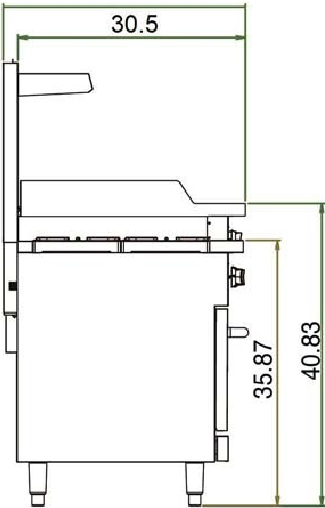
Side View
