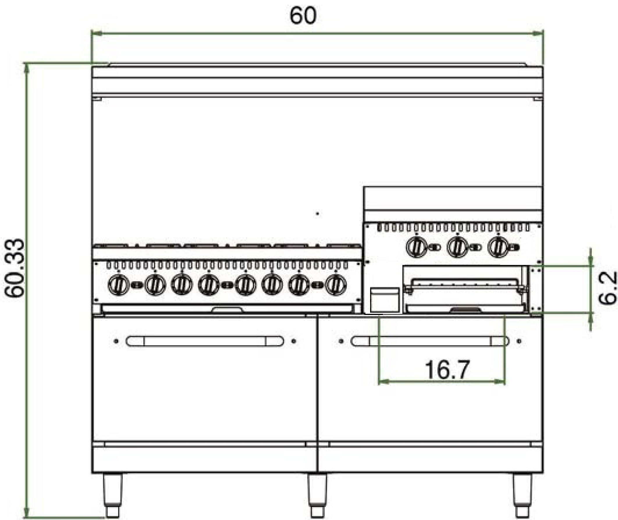
Front View
