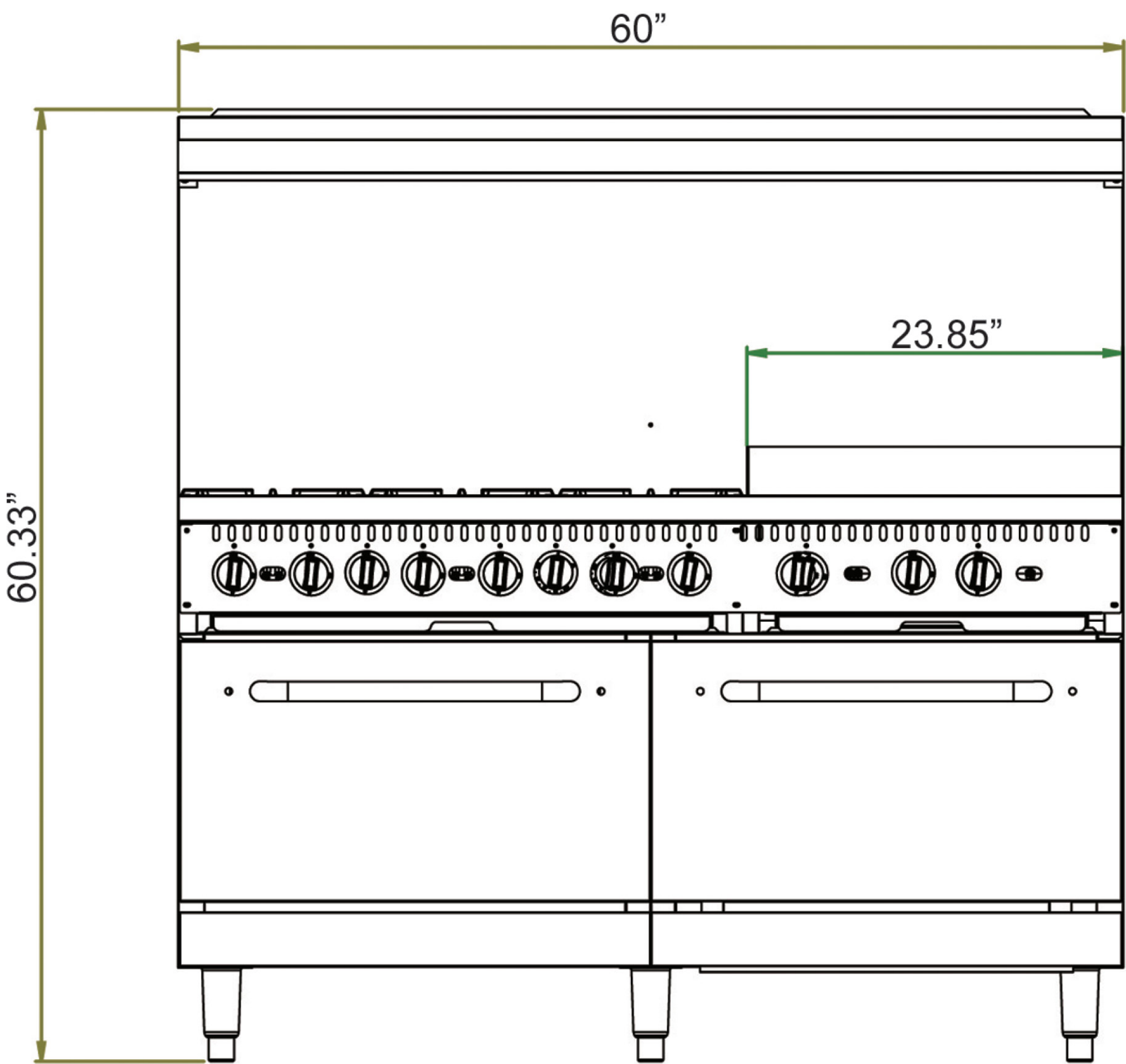
Front View
