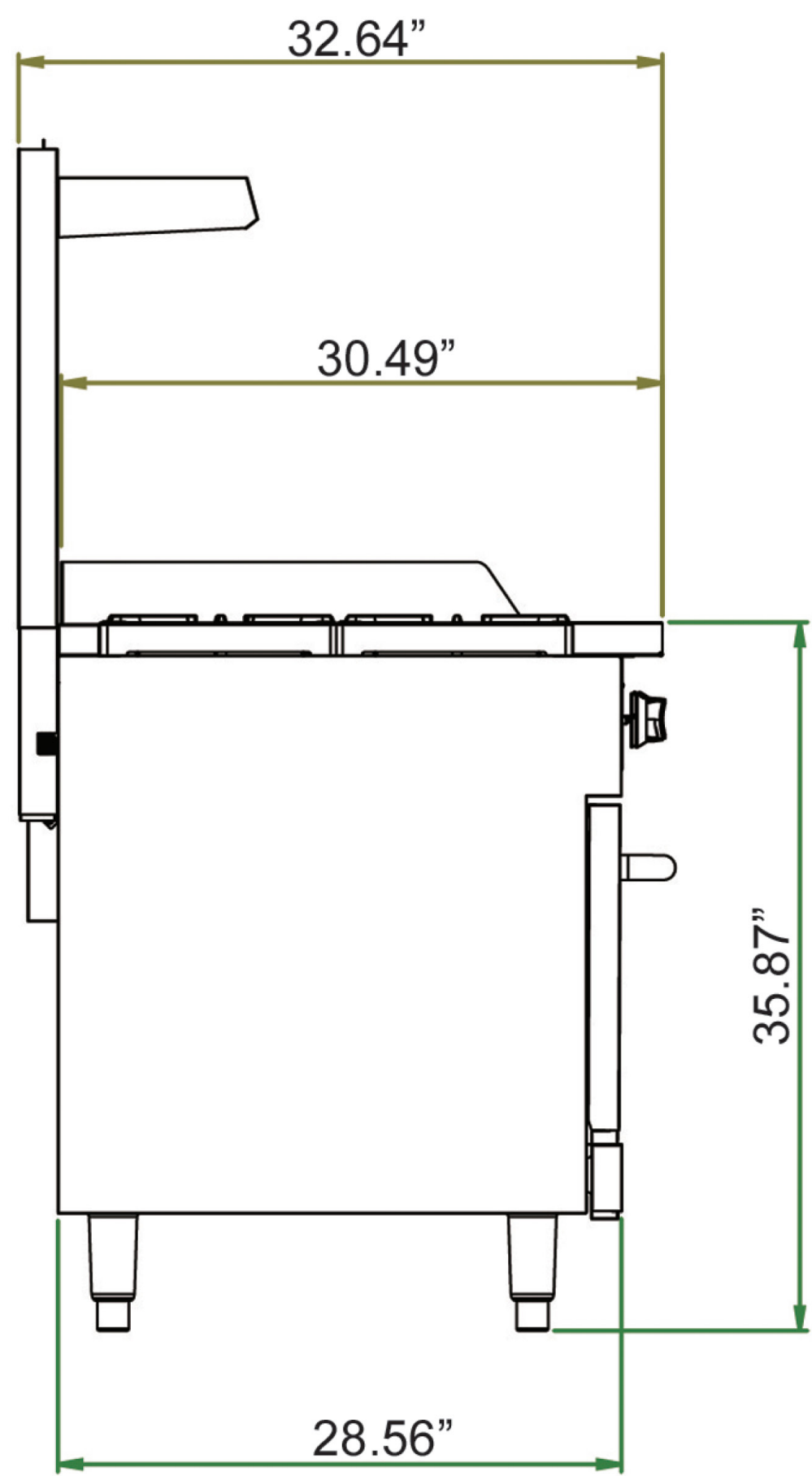
Side View
