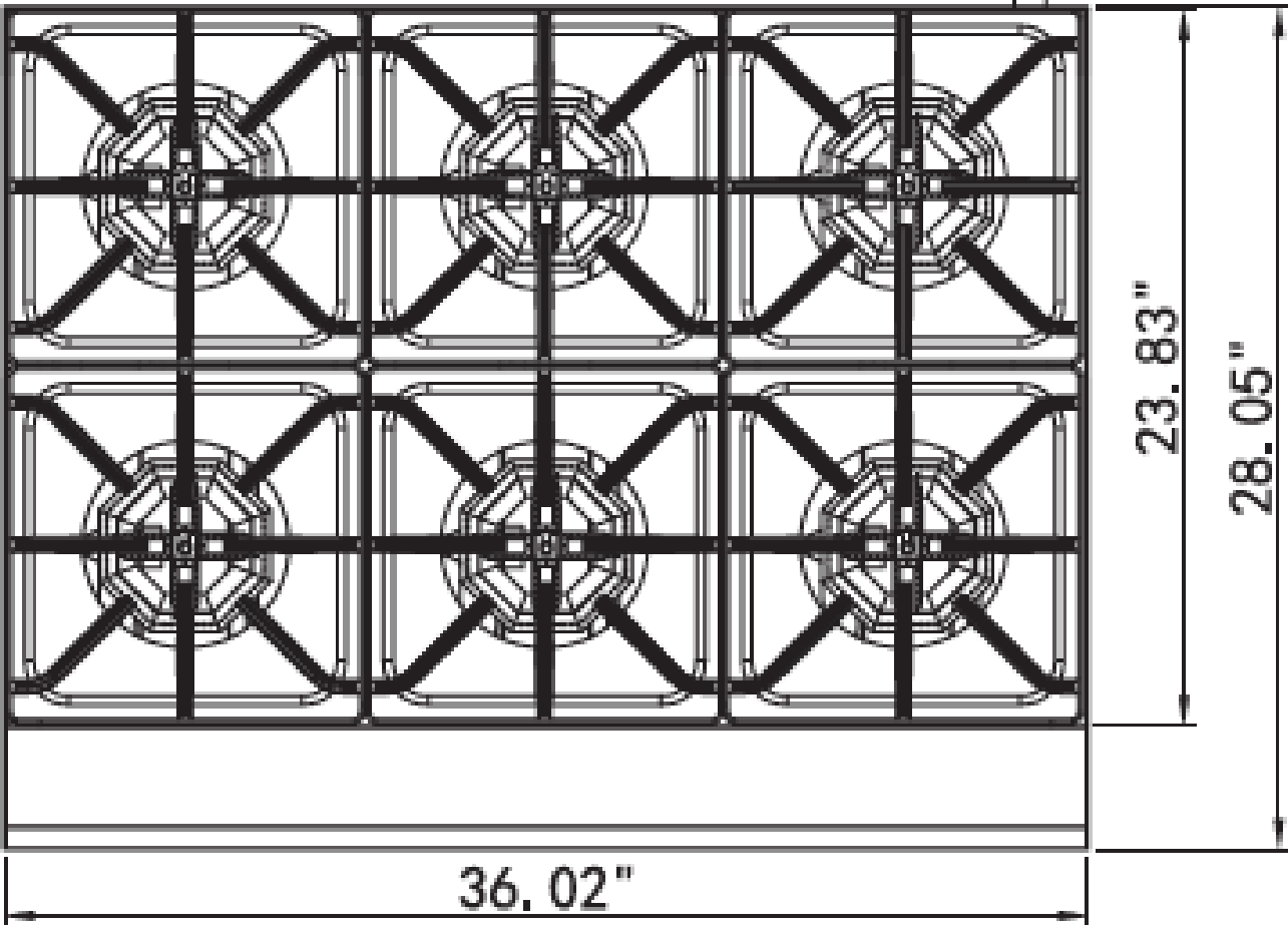
MHP36 - Top View
