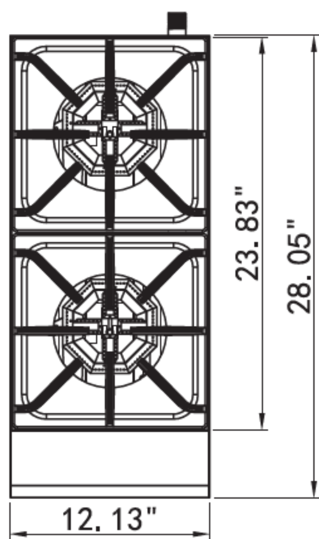
MHP12- Top View
