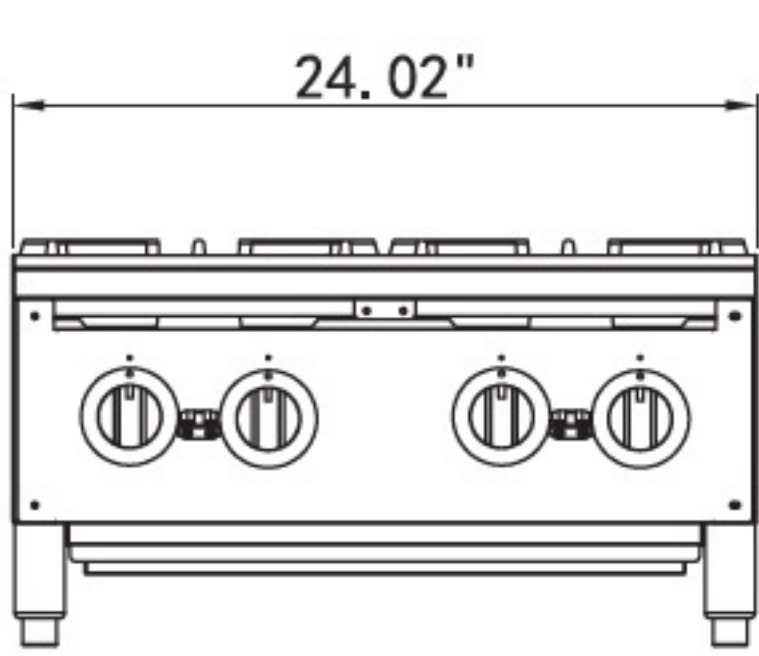
MHP24 - Front View
