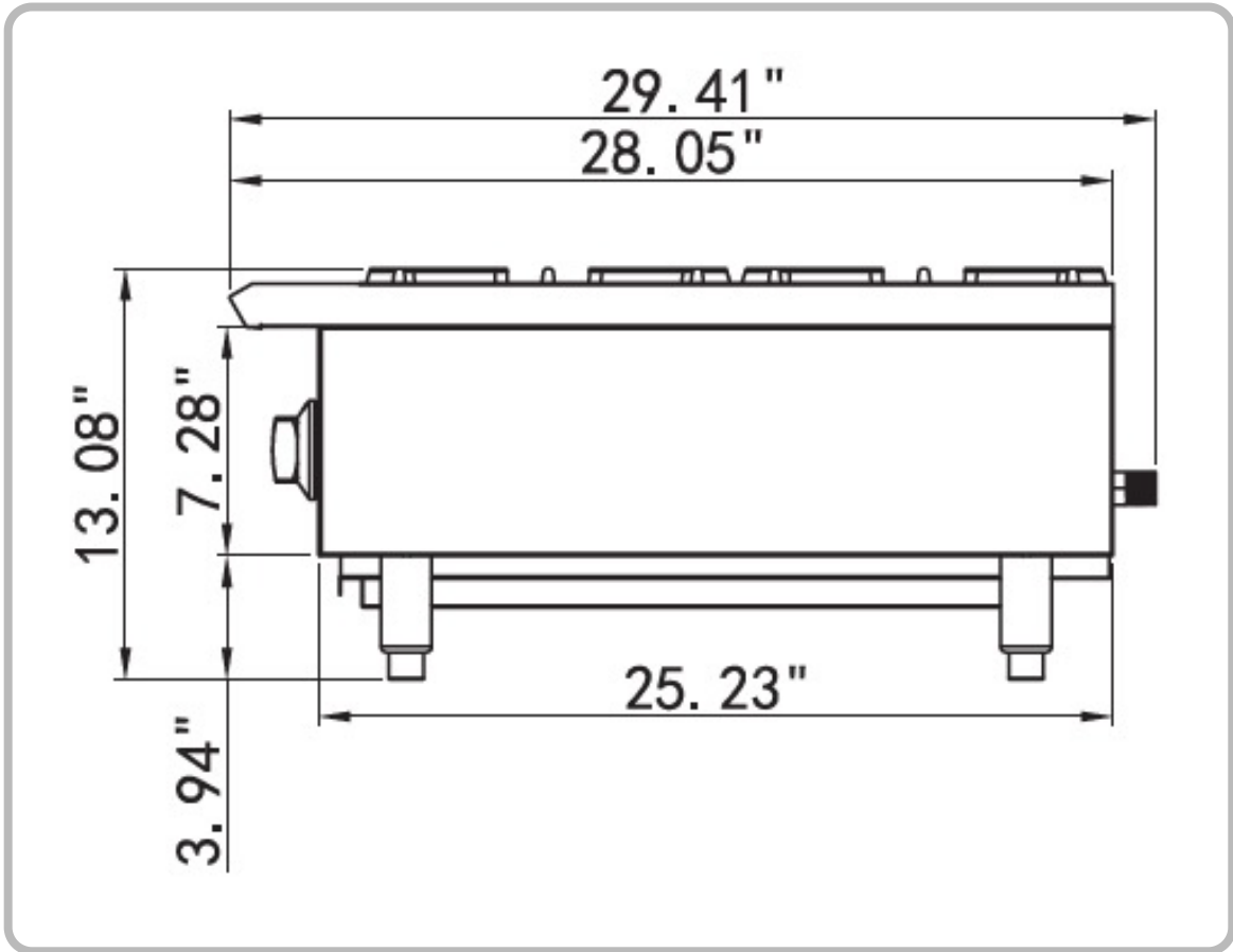
Side Views
