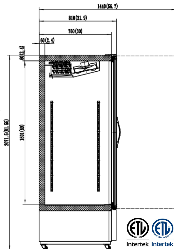
SIDE VIEW
