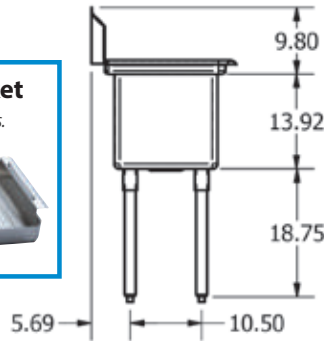
PROFILE DRAWING
