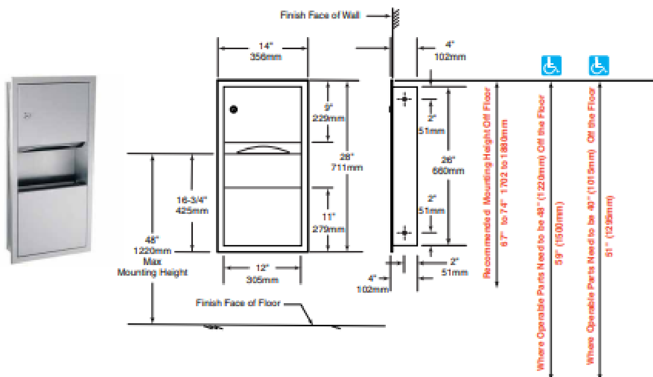
TW-3FS with 4" (102mm) skirt for surface-mounting
