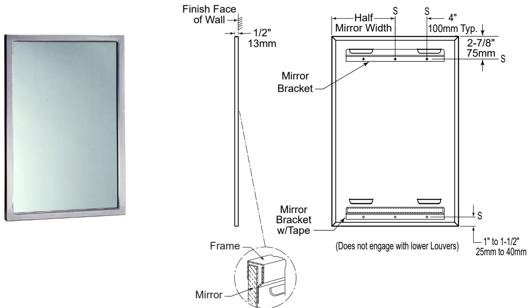
STANDARD A-SERIES MIRRORS
