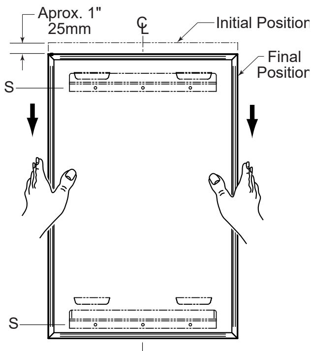
"S2" TAB DESIGN (Front View)
