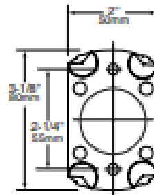
Snap Flange
