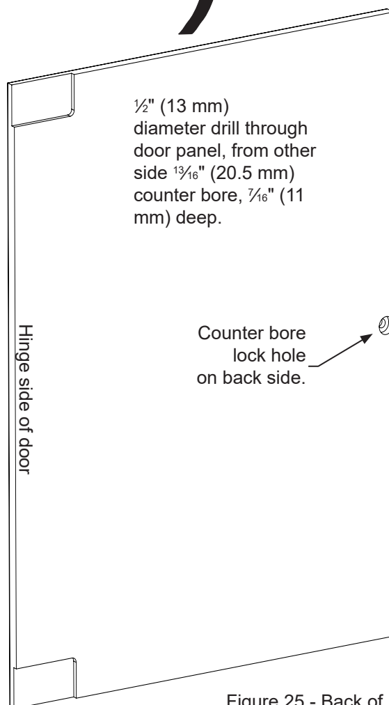
Figure 25 - Back of Panel
