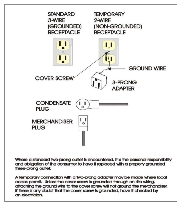
Figure 1: Grounding
