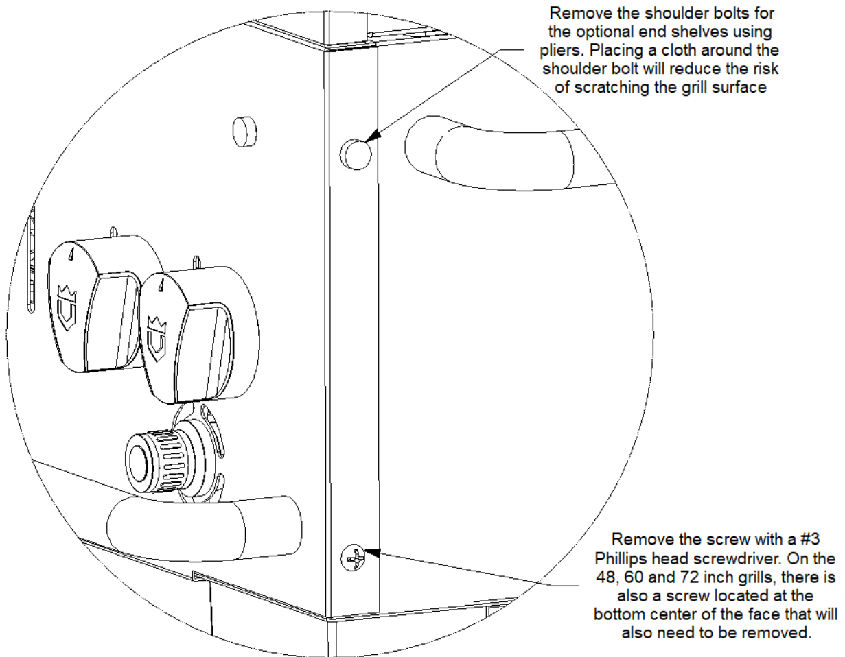
FIGURE 19. FACE REMOVAL
