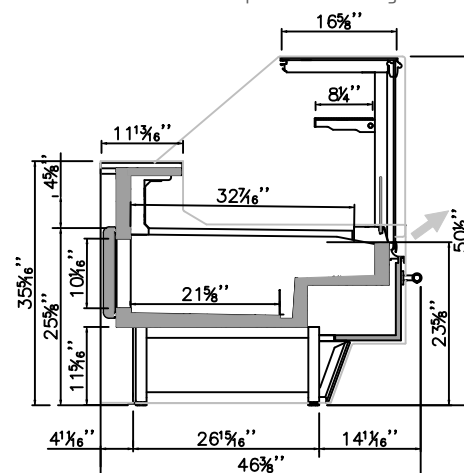
RCP Technical plan: With Storage
