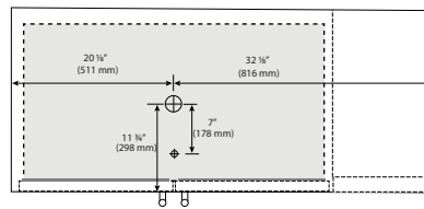
Tower 2 3/4" (70 mm)/Drain 1" (25 mm) Location
