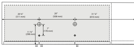
Tower 2 3/4" (70 mm)/Drain 1" (25 mm) Location
