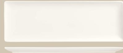
16" x 5½" Plate No. SL-22C H \frac{3}{4} 1 doz./25# • .6 cu. ft.
