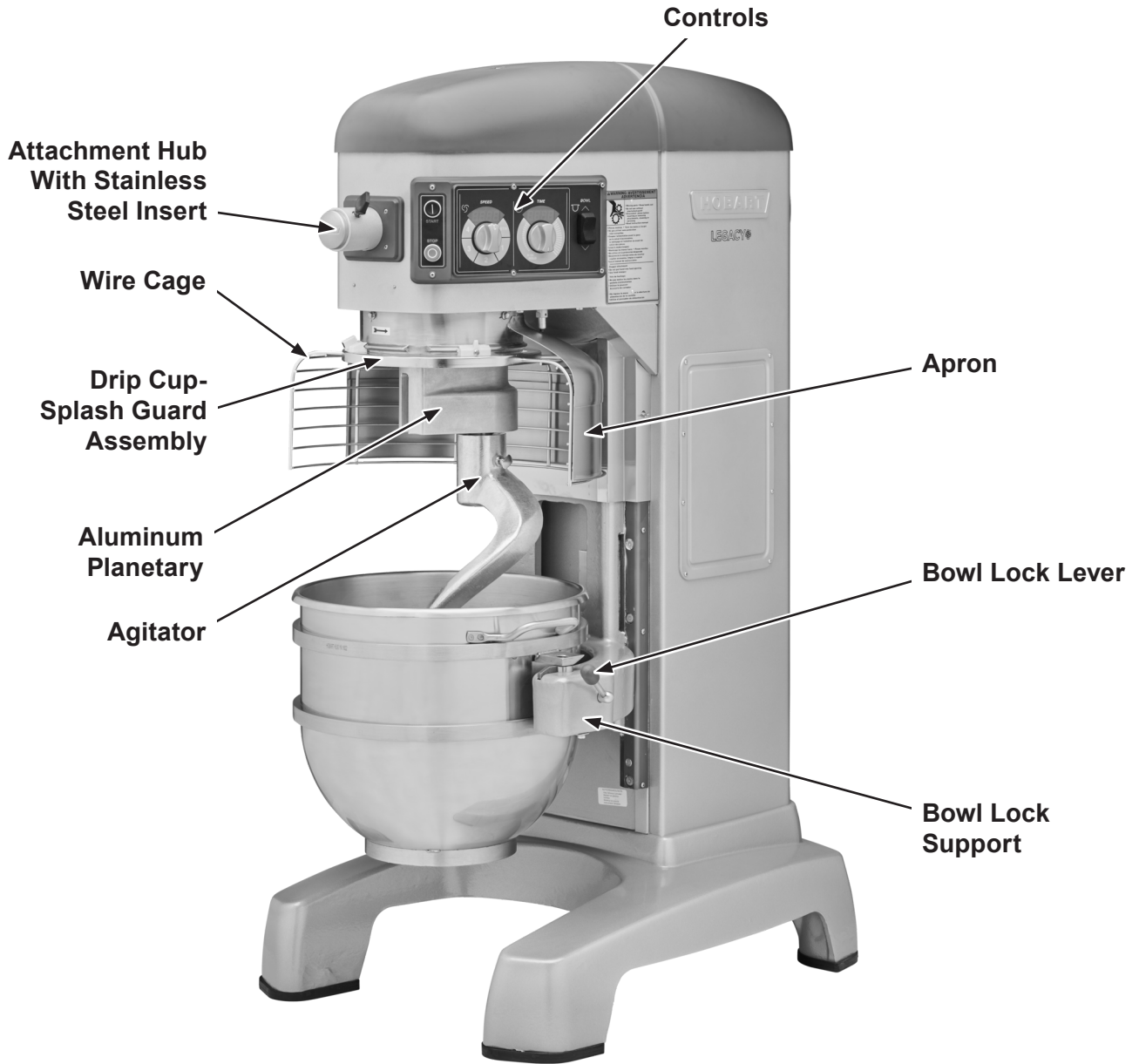
60-Quart Mixer
