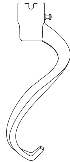
“ED” Dough Arm
