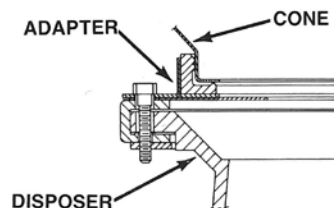
ADAPTER #ML-31161 Retains a special seal which is compressed against a Type #5 Cone.
