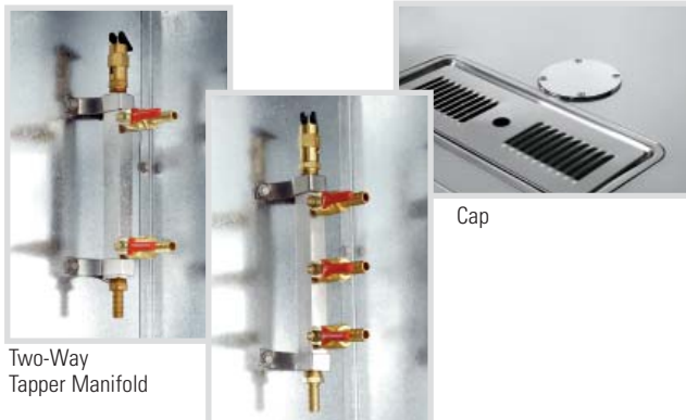
Three-Way Tapper Manifold
