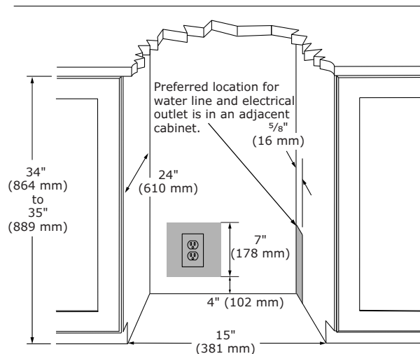
Cabinet Cut-Out
