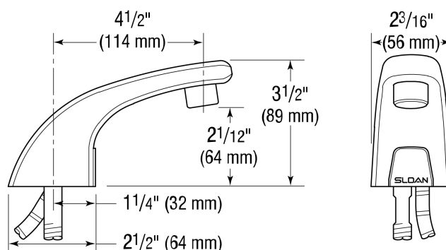
Variation not shown: 4" Trim Plate
