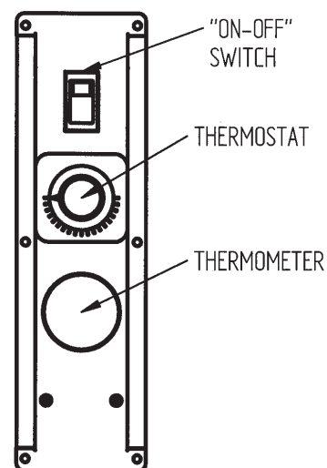
Figure 1 Control Panel
