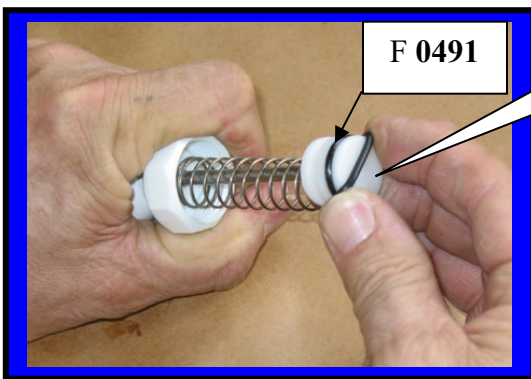
Installing Plunger Assembly into Faucet body
