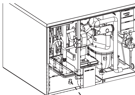
Fig. 23 Drain Plug
