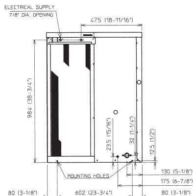
AIR-COOLED
