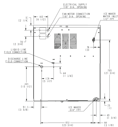
REMOTE AIR-COOLED
