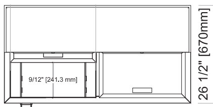
CC50(-S) Plan View
