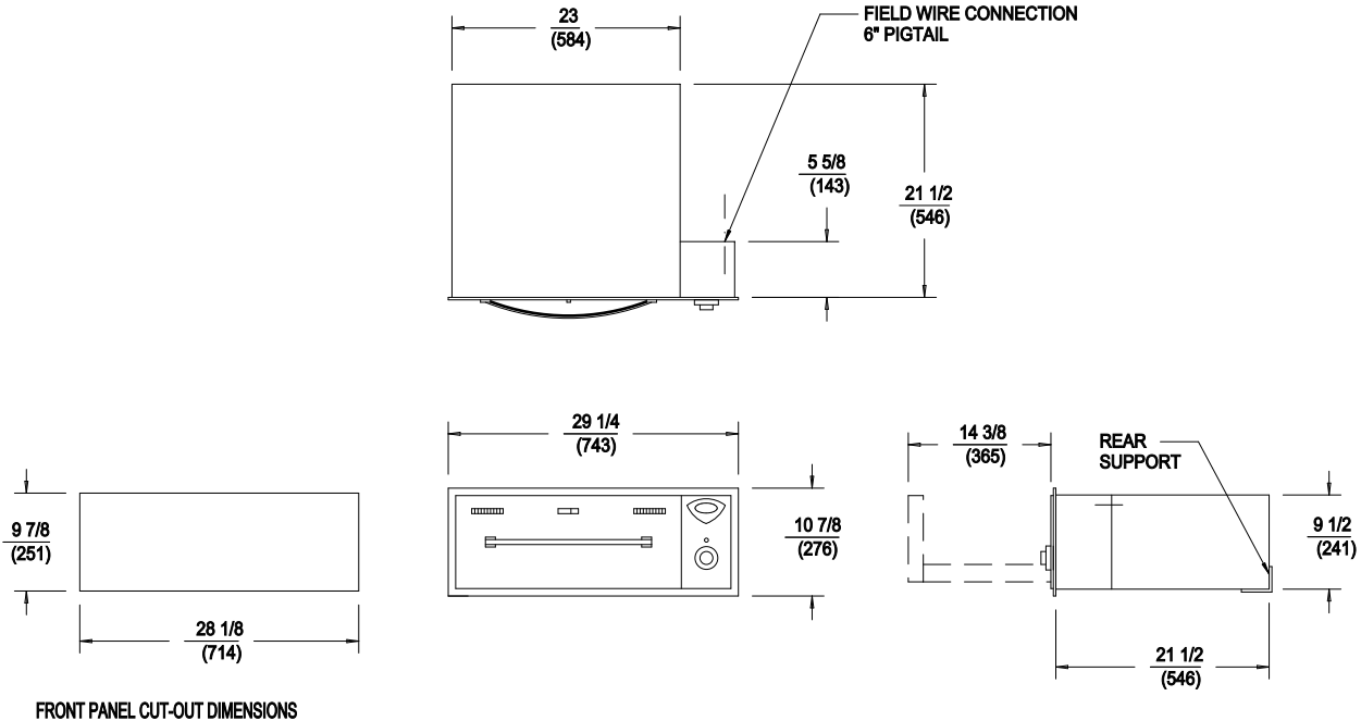
FRONT PANEL CUT-OUT DIMENSIONS
