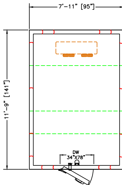
PLAN VIEW LEFT HINGE SELECT
