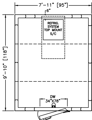
PLAN VIEW RIGHT HINGE SELECT
