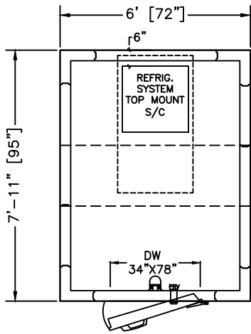
PLAN VIEW RIGHT HINGE SELECT
