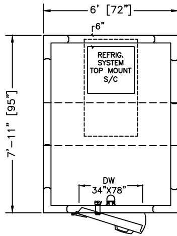
PLAN VIEW LEFT HINGE SELECT
