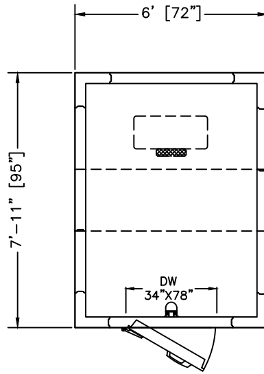
PLAN VIEW LEFT HINGE SELECT
