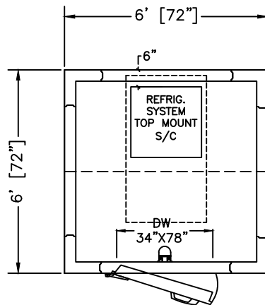
PLAN VIEW LEFT HINGE SELECT
