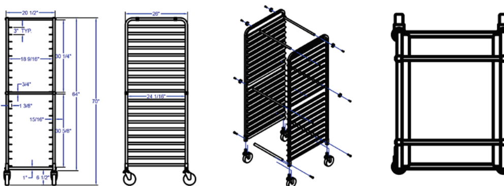
STANDARD MOBILE PAN RACK- ROUND TOP DESIGN
