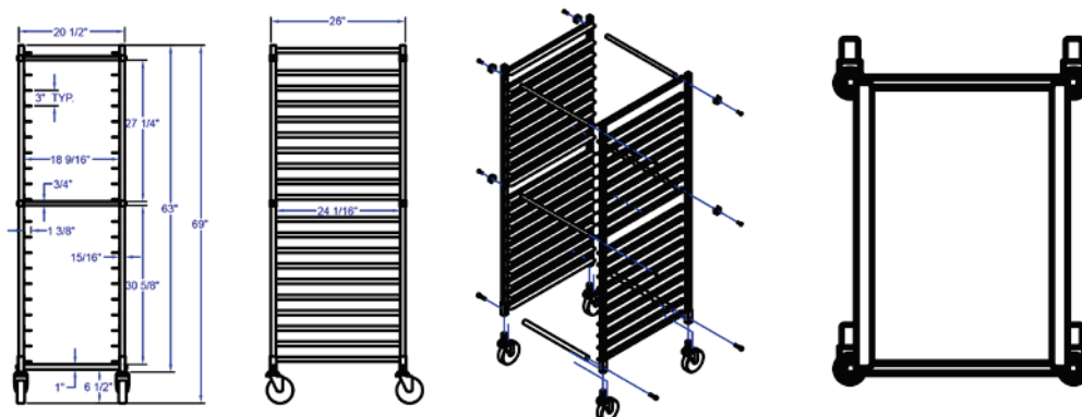
STANDARD MOBILE PAN RACK- SQUARE TOP DESIGN
