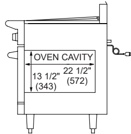
Side Convection Oven Base
