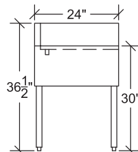
KR24 Corner Drainboard with Left Return
