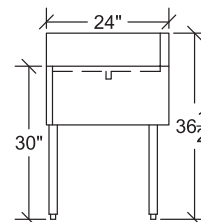
KR24 Corner Drainboard with Right Return
