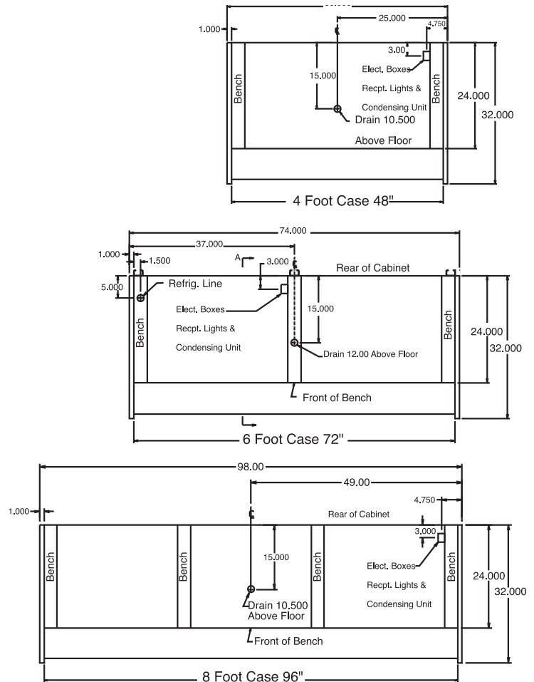
PLAN VIEWS
