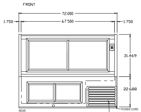
6' REAR VIEW
