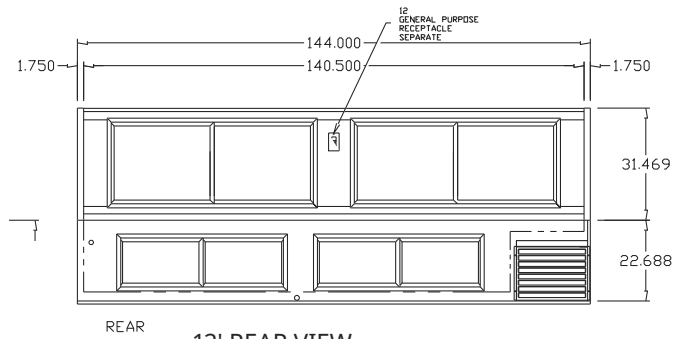
12' REAR VIEW
