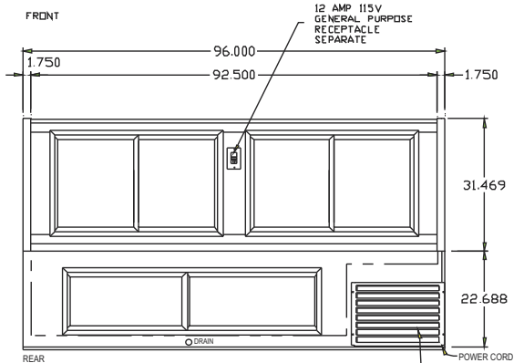
8' REAR VIEW
