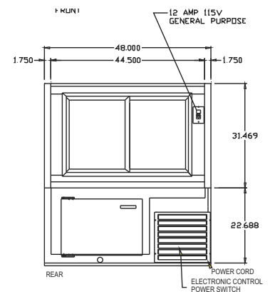
4' REAR VIEW
