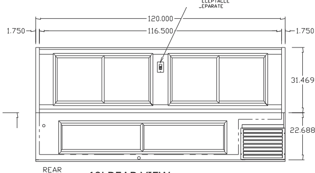
10' REAR VIEW
