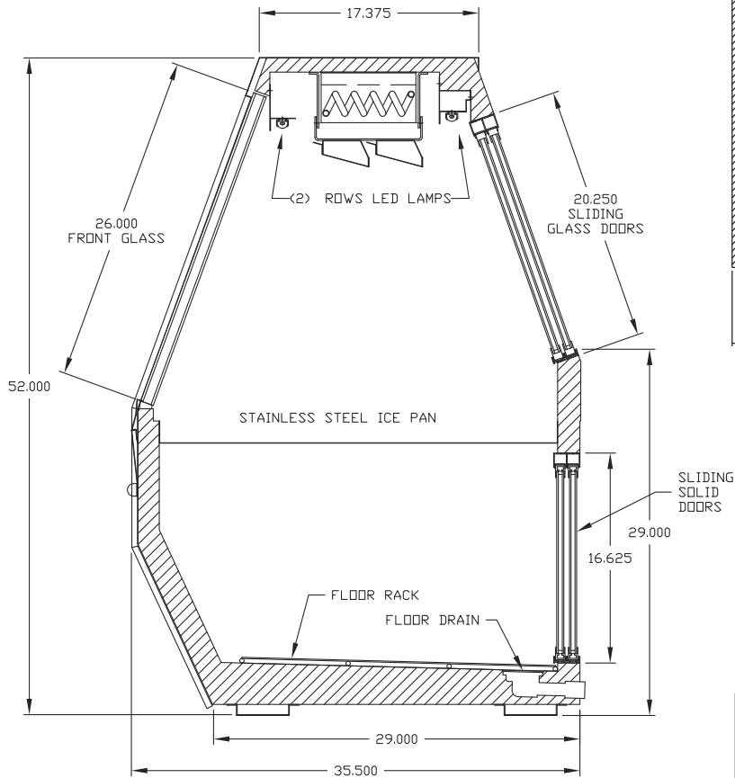
Cross Section
