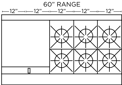
S60DD-2GL LINE: S-SERIES RANGE WIDTH: 60" WIDE BASE: (2) STANDARD OVENS TOP: 24" MANUAL GRIDDLE SECTIONS ON LEFT & (3) STANDARD BURNER SECTIONS
