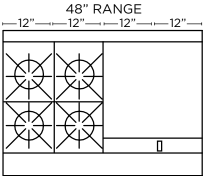
S48EE-2TR LINE: S-SERIES RANGE WIDTH: 48" WIDE BASE: (2) SPACE SAVER OVENS TOP: (4) STANDARD BURNERS ON LEFT & 24" THERMOSTATIC GRIDDLE ON RIGHT
