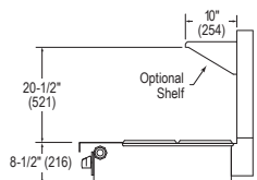
SIDE VIEW of MODULAR MODEL
