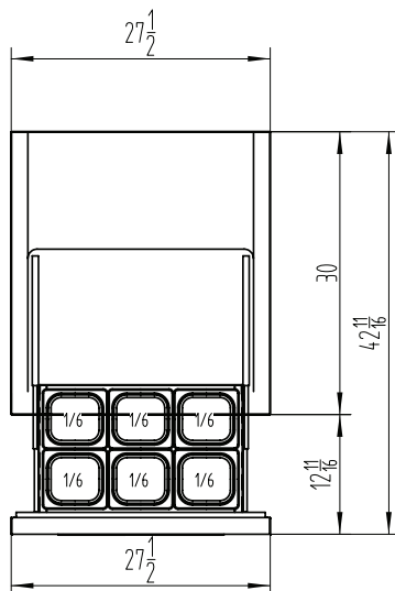
C-U27F-D-HC TOP VIEW
