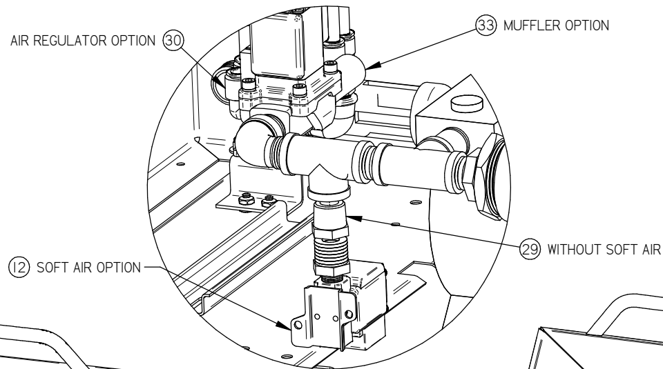
DETAIL C
