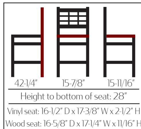
Walnut stain Wood Seat SL2163-1-WA
